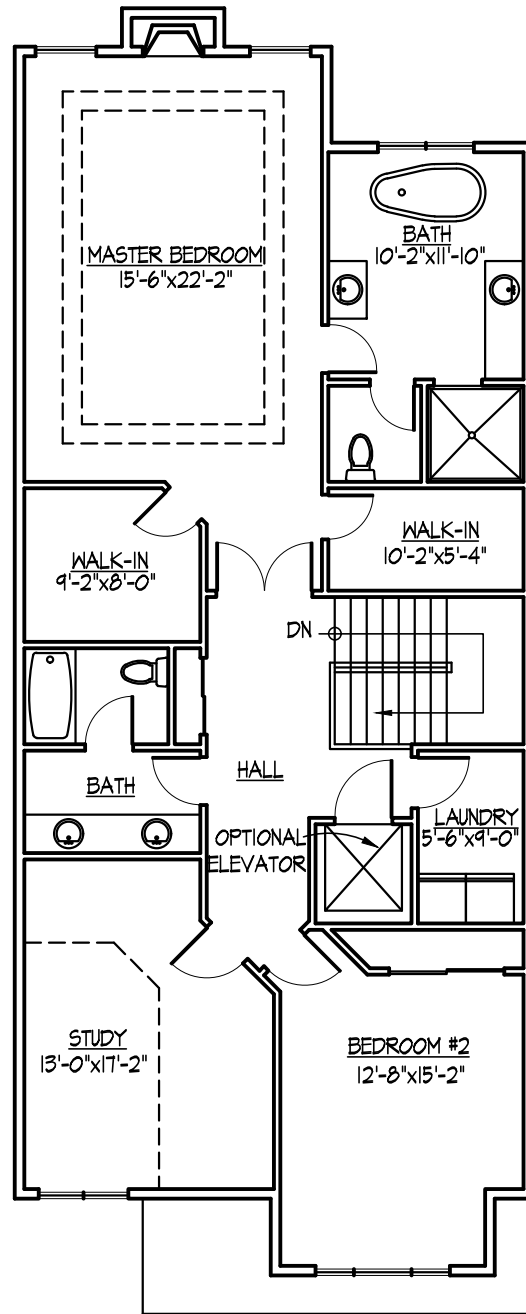
TYPICAL UPPER LEVEL PLAN NOT TO SCALE 1,535 S.F.
