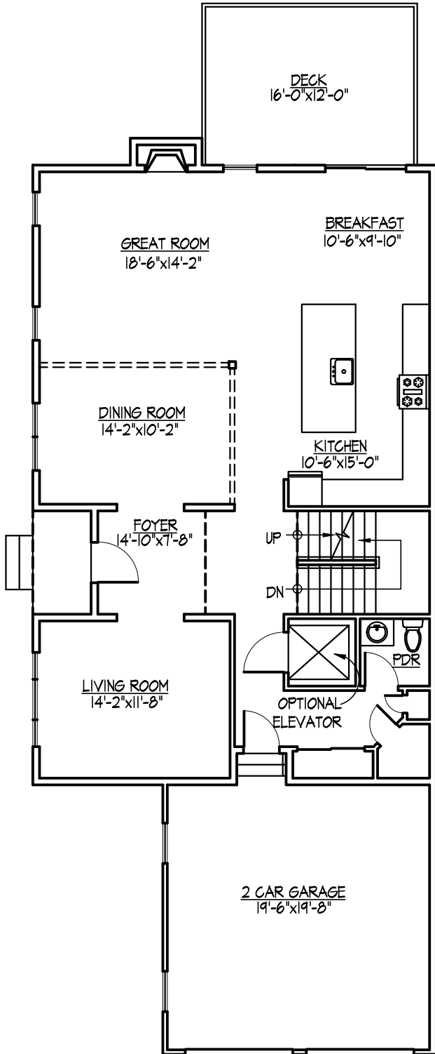
TYPICAL MAIN LEVEL PLAN
