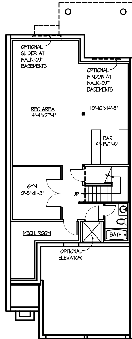
OPTIONAL WALK-OUT BASEMENT PLAN NOT TO SCALE
