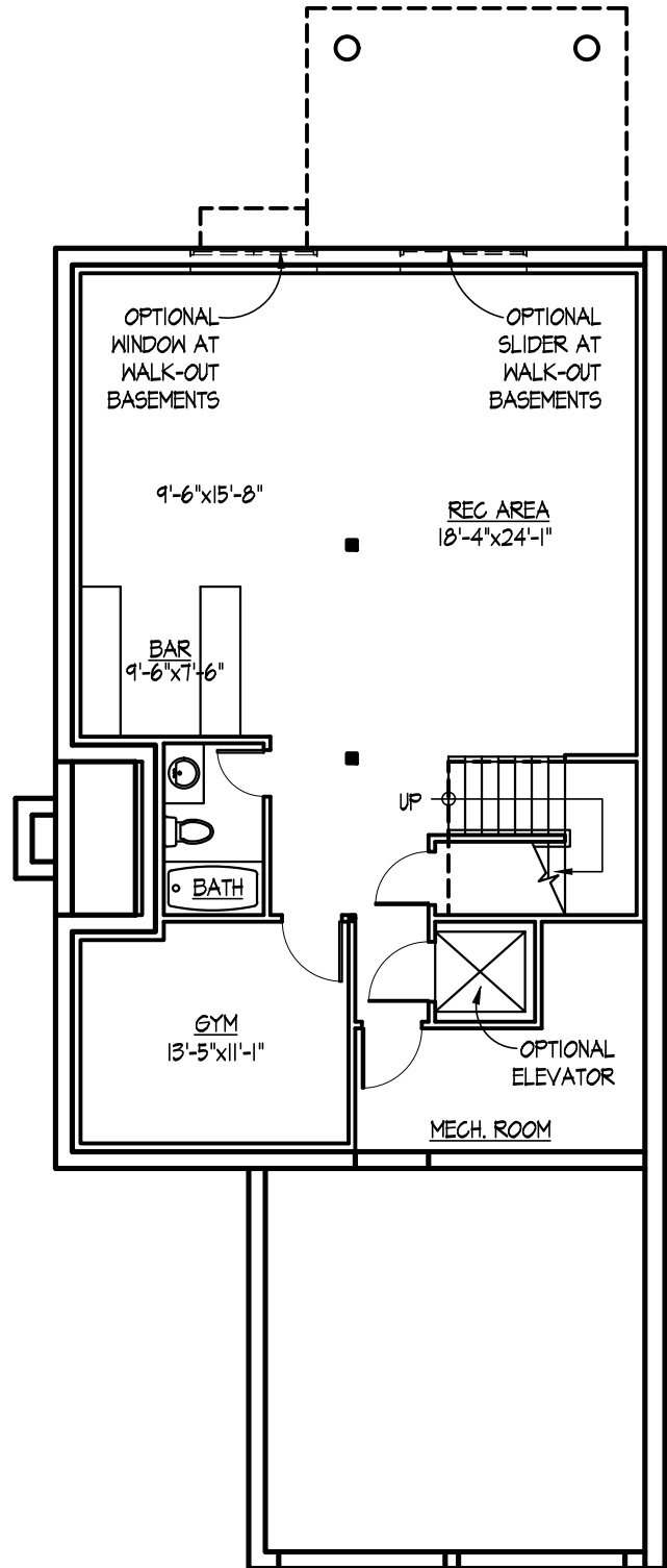
OPTIONAL BASEMENT PLAN NOT TO SCALE
