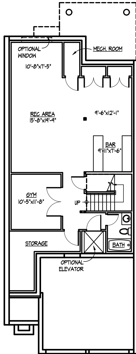
OPTIONAL BASEMENT PLAN NOT TO SCALE
