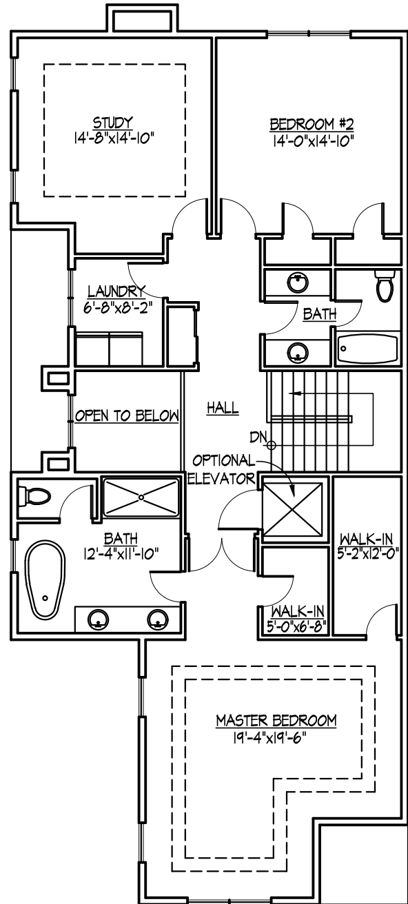
TYPICAL UPPER LEVEL PLAN
